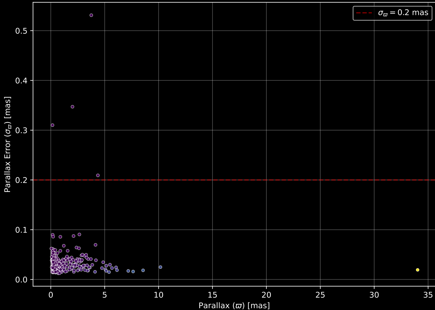
APOGEE DR17 Field: [180-08] Parallax Quality (n= 503)
