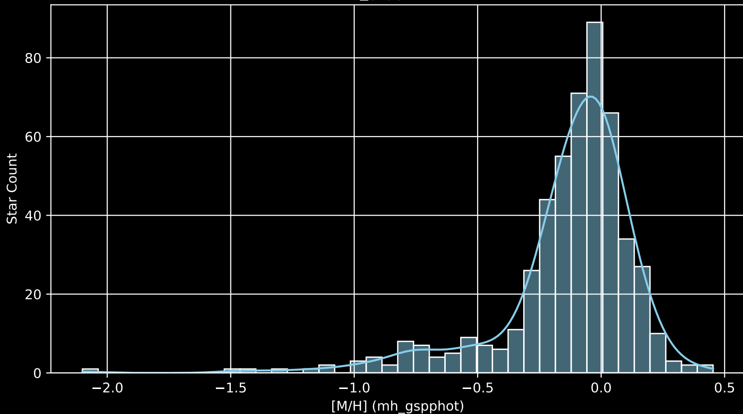
APOGEE DR17 Field: [180-08 [M/H] (mh_gspphot) (n= 502)
