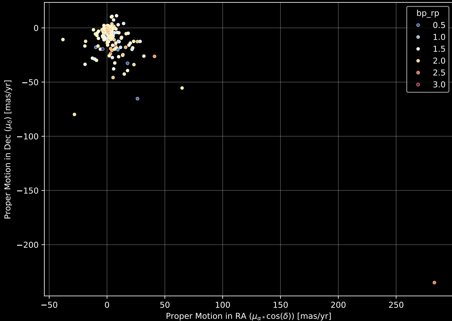
APOGEE DR17 Field: [180-08] Proper Motion Diagram (n= 503)
