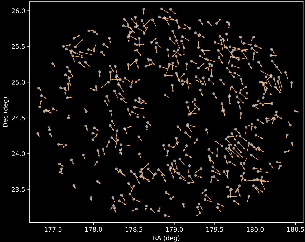
APOGEE DR17 Cluster 3 Proper Motion Vectors (n=381)
