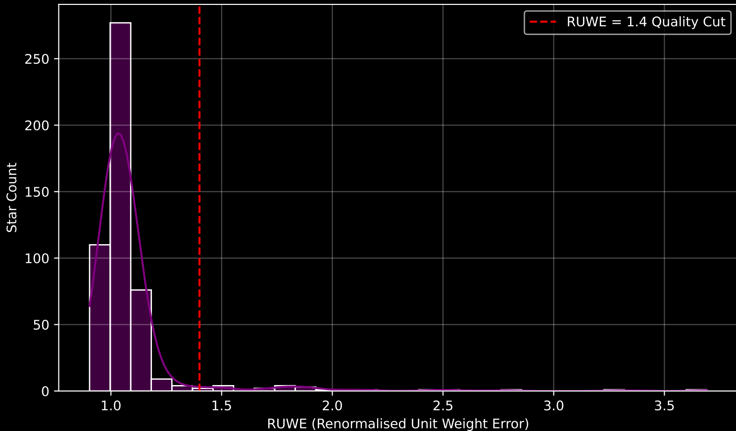
GAPOGEE DR17 Field [180-08] RUWE Distribution (n= 499)
