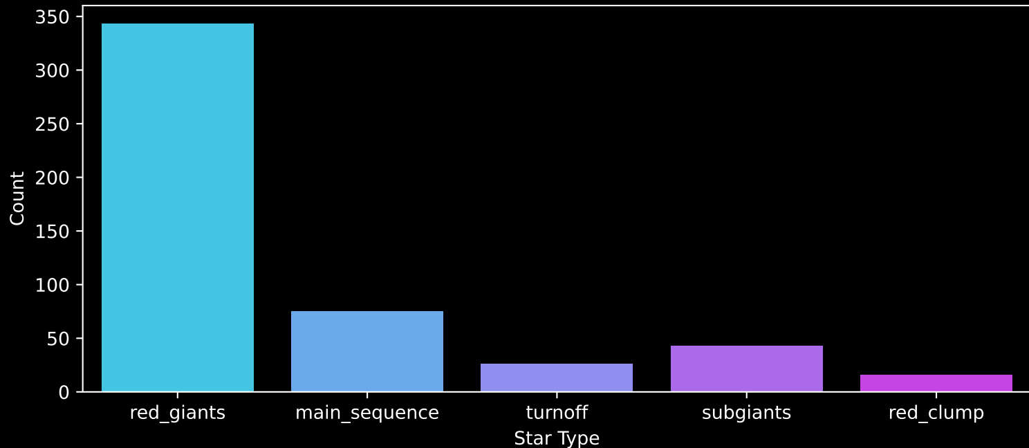
APOGEE DR17 Field: [180-08] Count plot of Star Type
